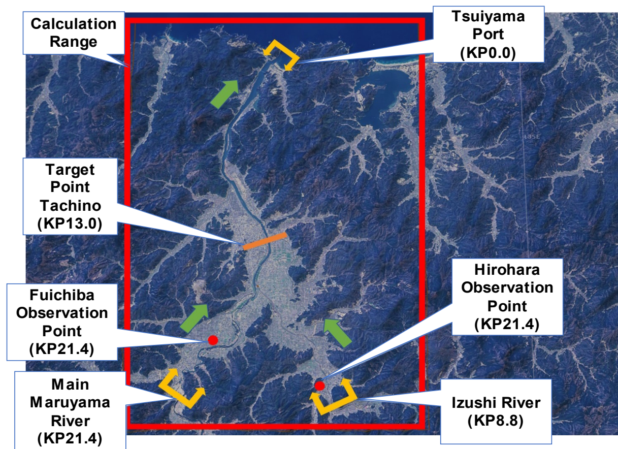
Fig. 2 Calculation Range
