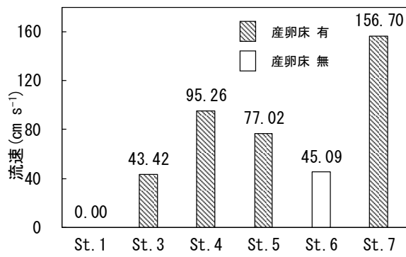
Fig. 21 Flow velocity at spawning redds (2018FY)
