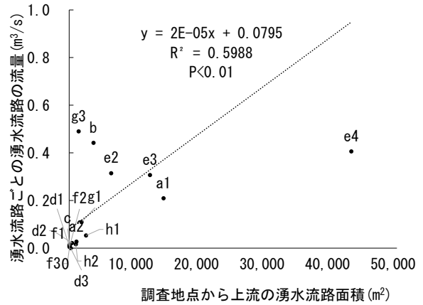
Fig. 44 Relations of discharge of spring channels to spring channel area of upstream from the survey point
