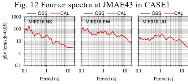
Fig. 12 Fourier spectra at JMAE43 in CASE1
