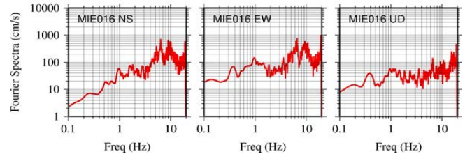
Fig. 15 Acceleration waveforms at MIE016 in CASE2
