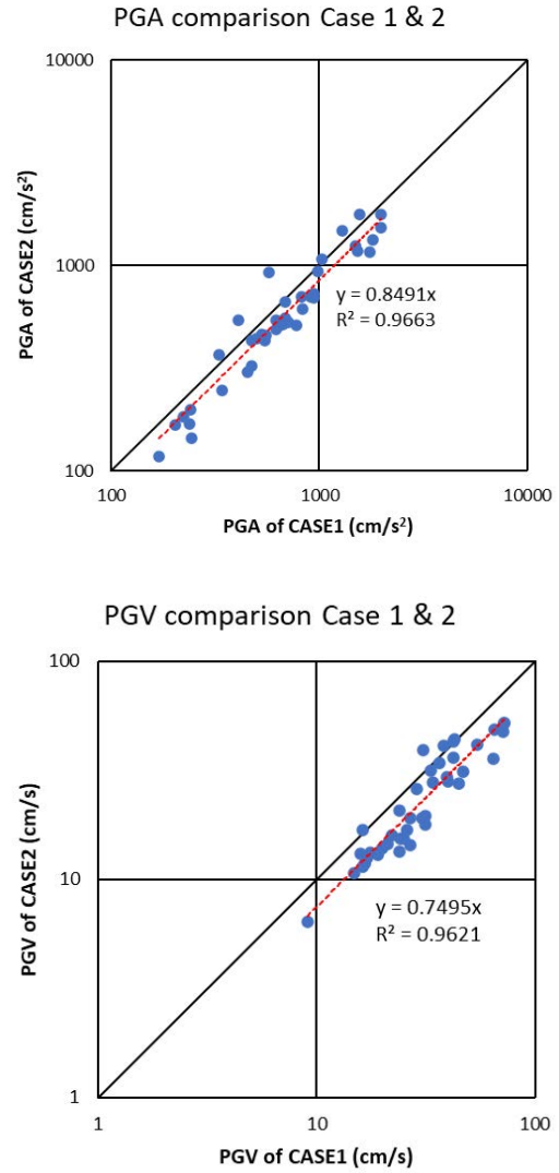
Fig. 22 Comparisons of PGA and PGV for the calculated synthetics with slip variations (CASE1) and without slip variations (CASE2).
