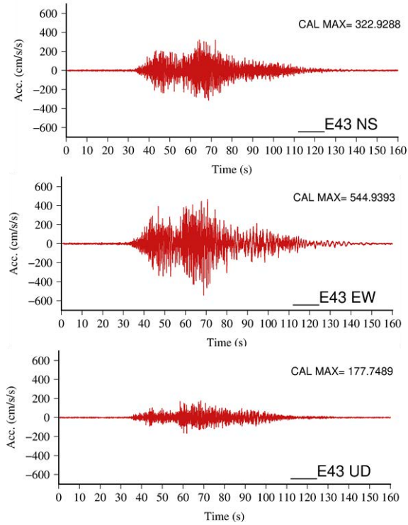
Fig. 8 Acceleration waveforms at JMAE43 in CASE1
