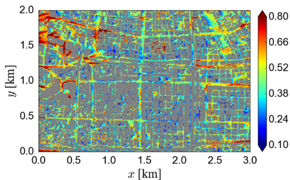
Fig. 11 The horizontal distribution of the ratio of the maximum instantaneous surface wind speed to the wind speed at the reference height in Osaka City
