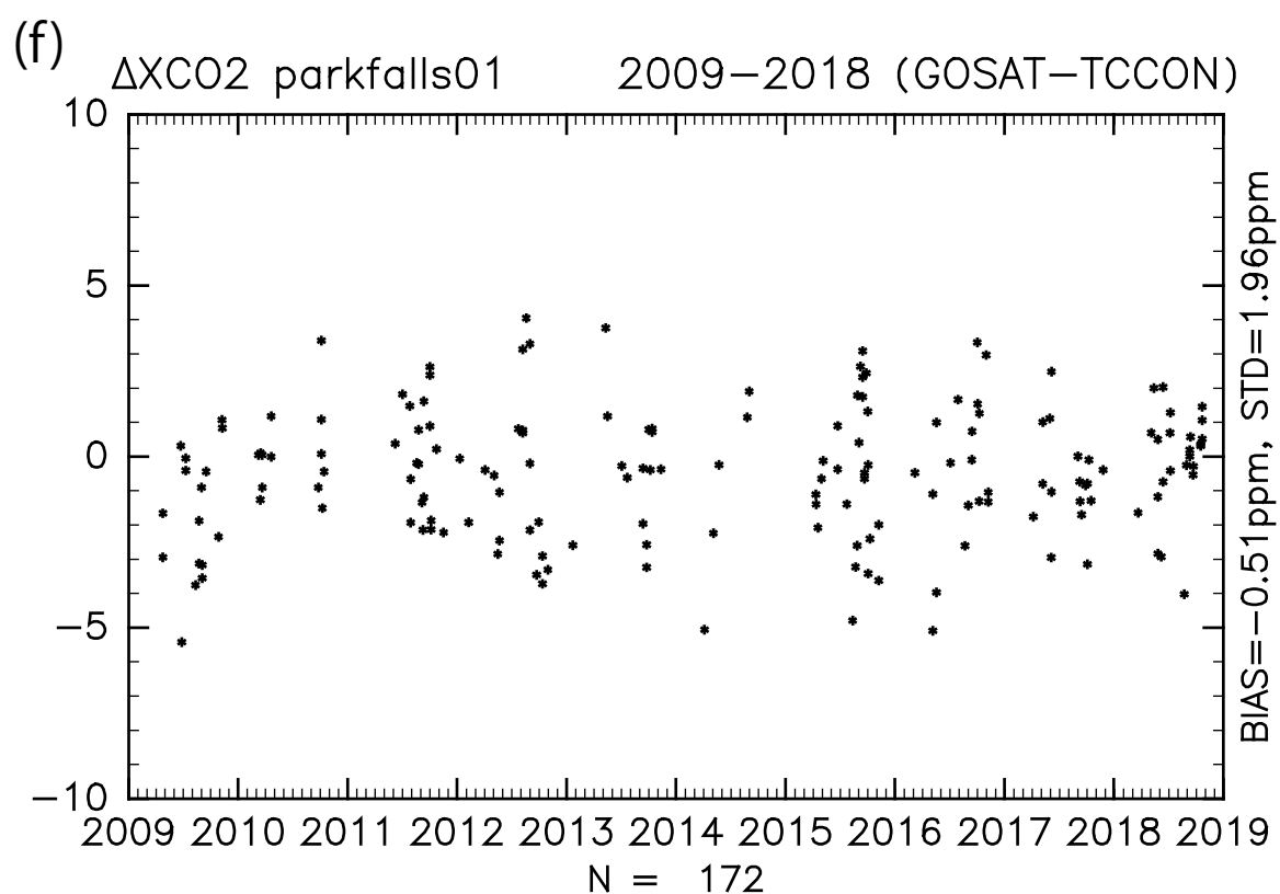
Fig. 1(continued) (e) XCO 2 and (f) \Delta XCO 2 at Park Falls, same as (a) and (b).
