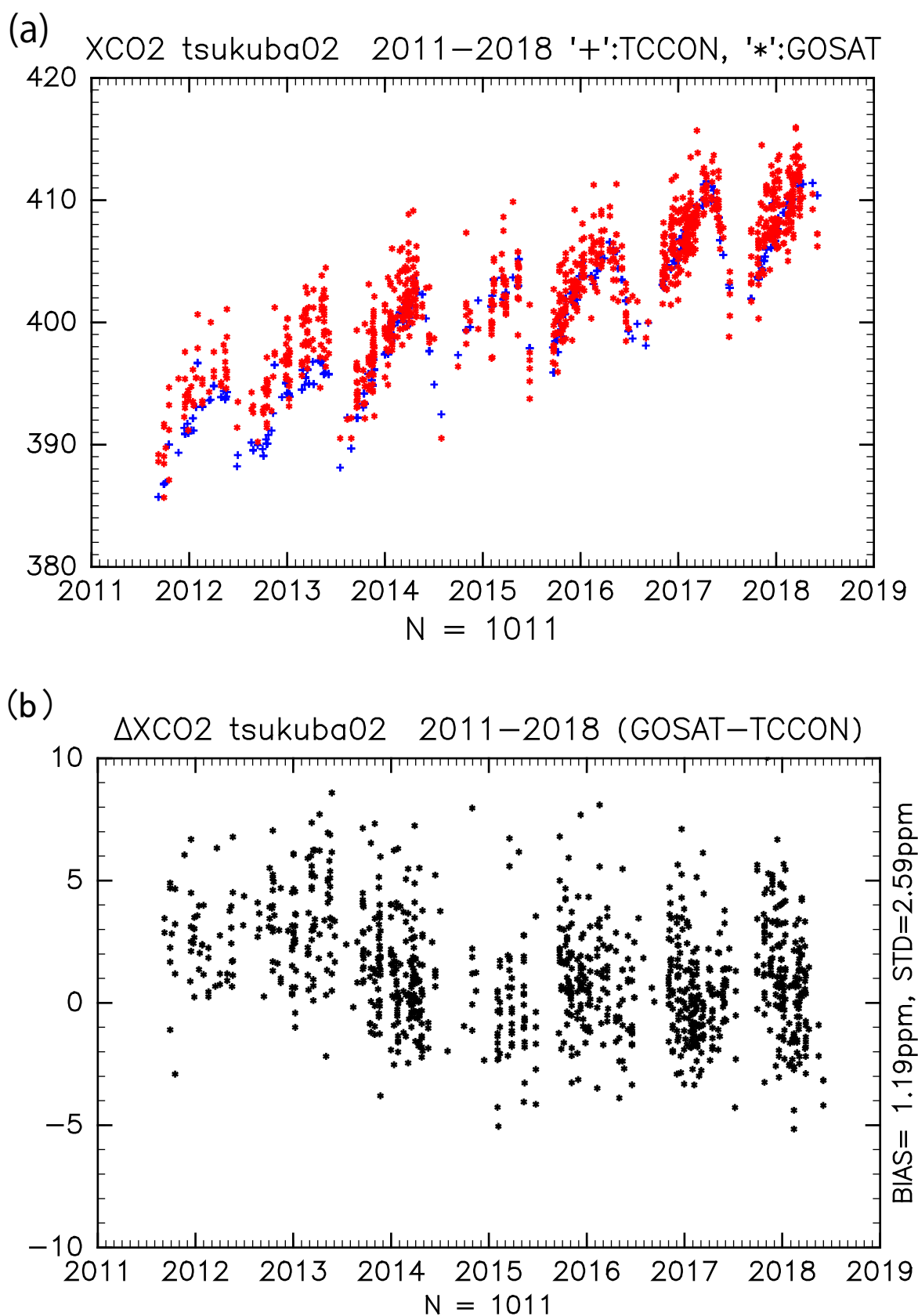
Fig 1 (a) XCO 2 of GOSAT FTS SWIR L2 CO 2 V02.72 product (the red '*' marks) and TCCON GGG2014 data (the blue '+' marks) at Tsukuba. N is number of plots of GOSAT and TCCON data respectively. (b) \Delta XCO 2 (difference of XCO 2 between GOSAT and TCCON data) at Tsukuba. BIAS is average of \Delta XCO 2 , and STD is root mean square of \Delta XCO 2 .
