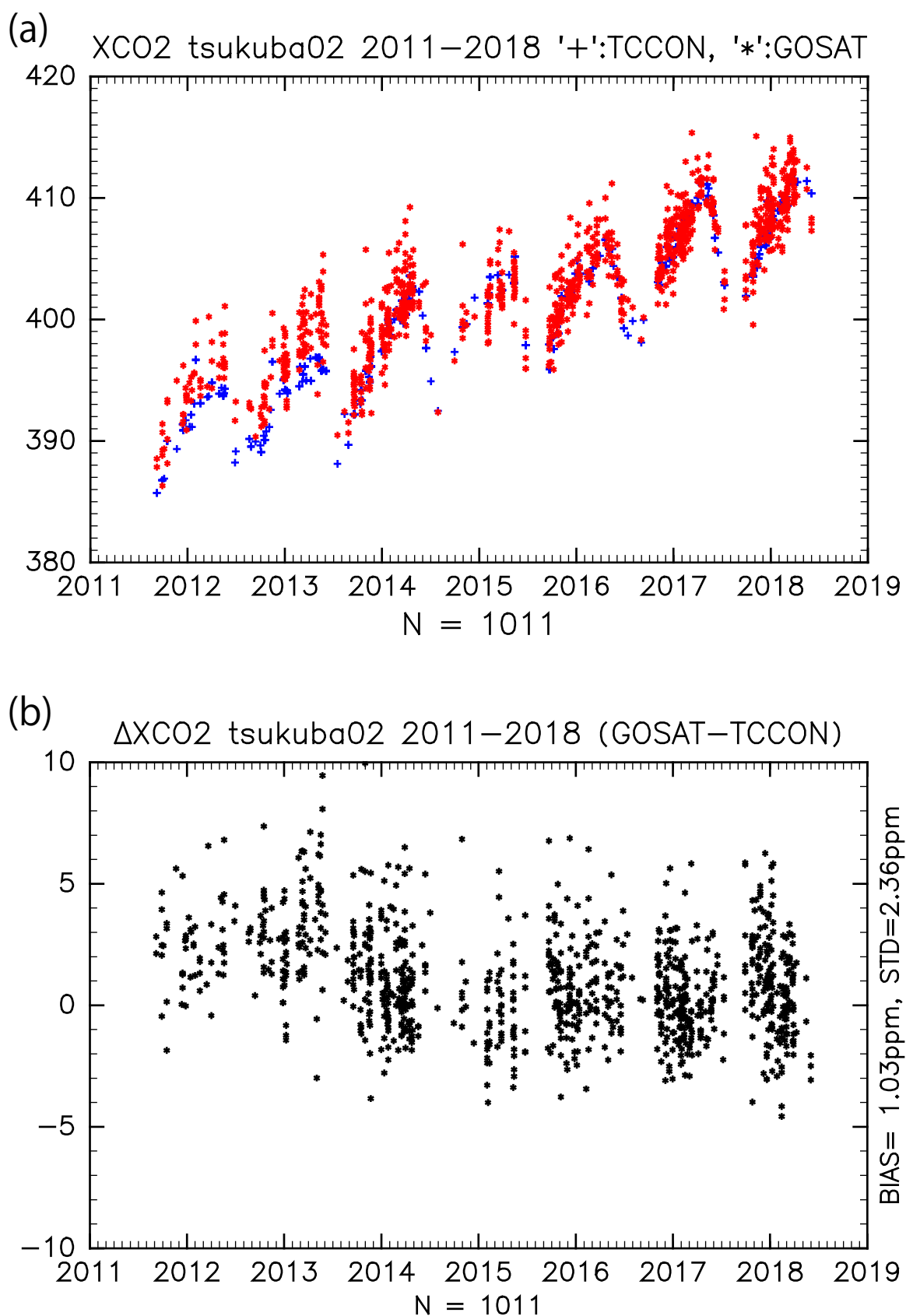
Fig 3 (a) XCO 2 of GOSAT FTS SWIR L2 CO 2 V02.75 product (the red '*' marks) and TCCON GGG2014 data (the blue '+' marks) at Tsukuba, same as Fig. 1(a). (b) \Delta XCO 2 at Tsukuba, same as Fig. 1(b).
