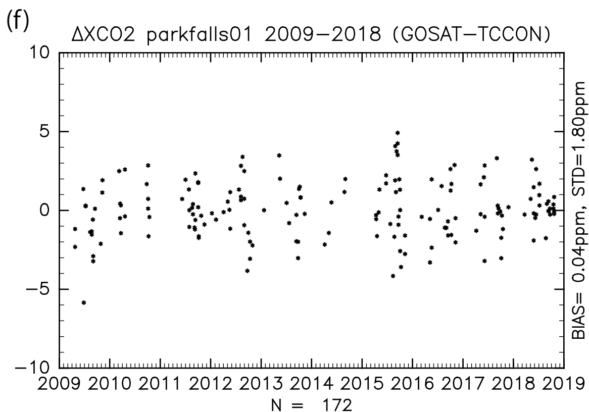
Fig. 3(continued) (e) XCO 2 and (f) \Delta XCO 2 at Park Falls, same as (a) and (b).
