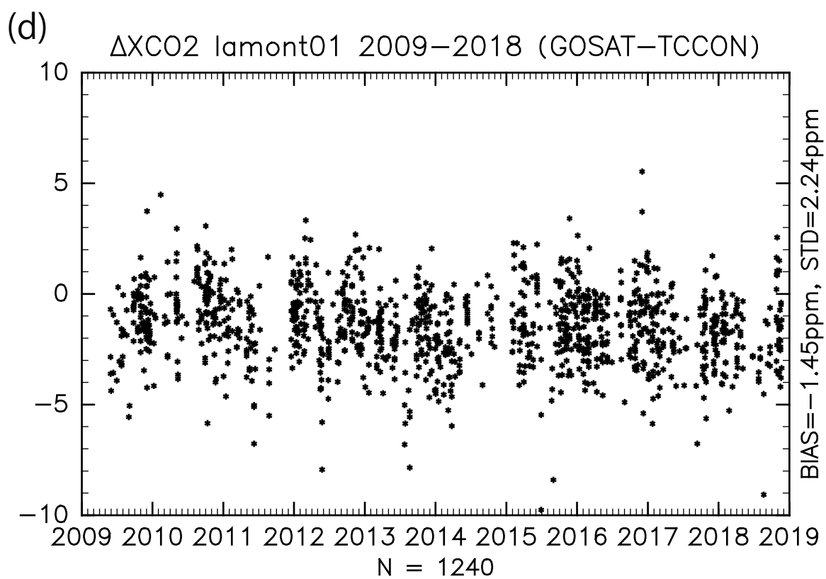
Fig. 1(continued) (c) XCO 2 and (d) \Delta XCO 2 at Lamont, same as (a) and (b).
