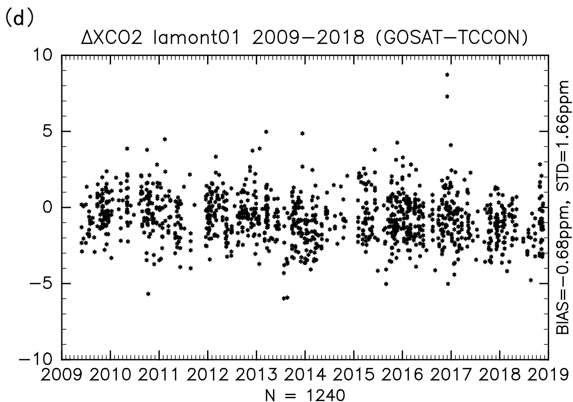
Fig. 3(continued) (c) XCO 2 and (d) \Delta XCO 2 at Lamont, same as (a) and (b).
