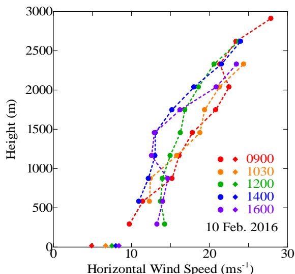
Fig. 5 Vertical profiles of horizontal wind speed observed by a wind profiler at Nagoya Local Meteorological Observatory on 10 February 2016. Horizontal wind speeds measured by a windmill anemometer at the surface are also shown.
