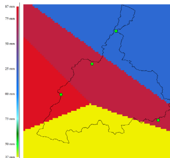
Fig. 3 Measured rainfall for Gonu 2007 event in W. Samail
