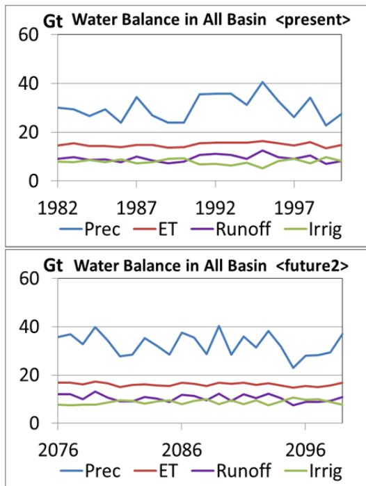
Fig. 7 Water balance in whole basin.
