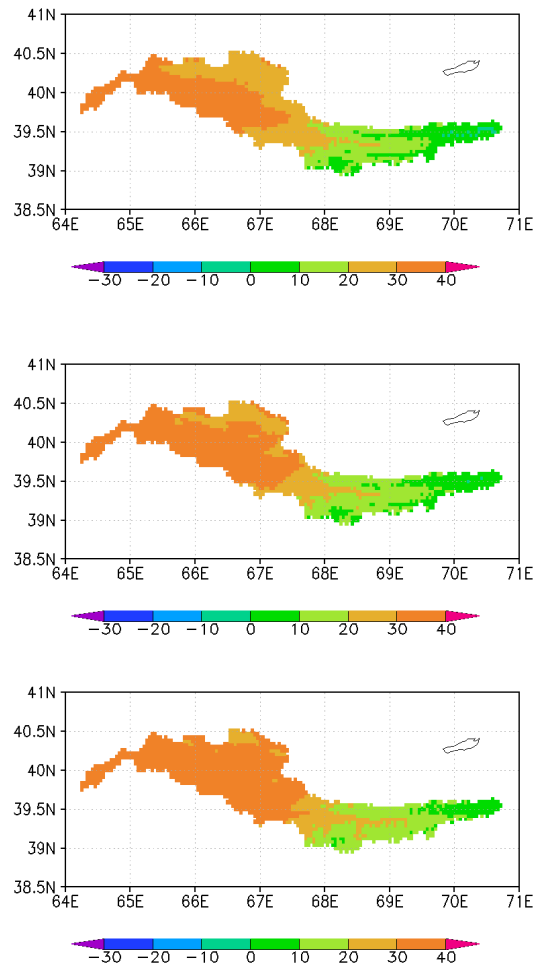
Fig. 8 Comparison of the temperatures in July. a) present; b) average for 2030-2050; c) future average 2050-2099
