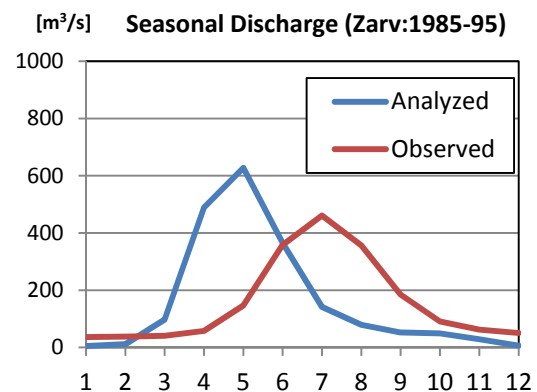
Fig. 5 Simulation of the discharge within a year
