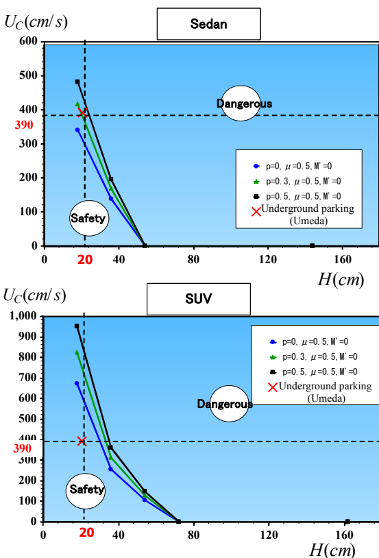
Fig.10 Incipient velocity for flooded car (Real scale)
