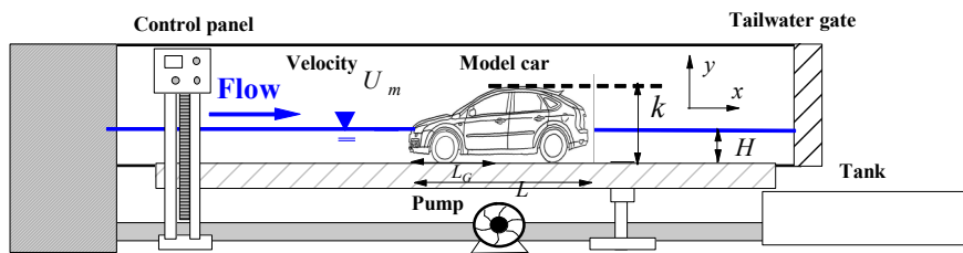
Fig.2 Experimental setup(Flooded car)
