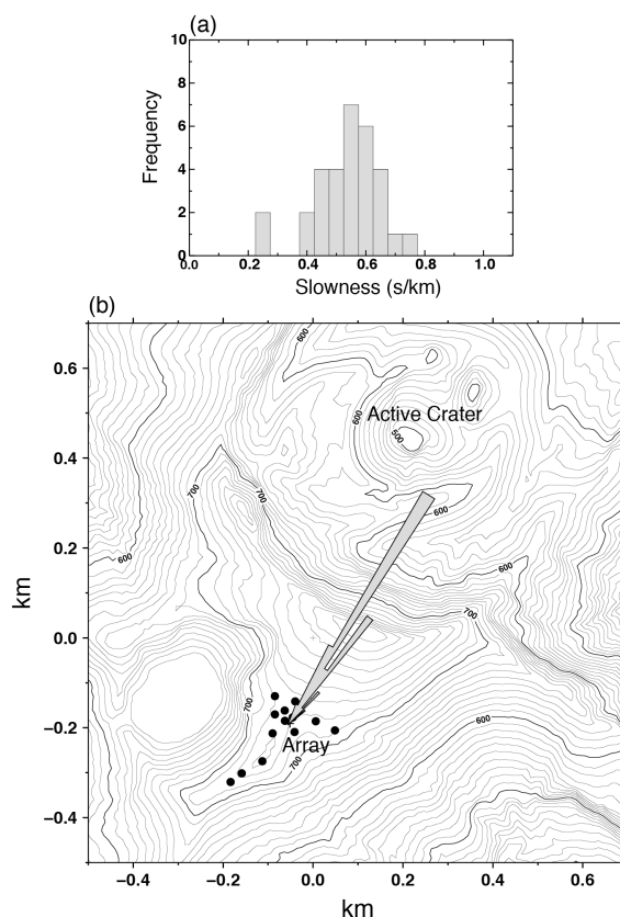
Fig. 6 (a) Frequency histogram of the apparent slowness values for the maximum semblance values in the S-wave time window of the 30 explosion earthquakes. (b) Rose diagram of the back azimuths of the S-wave time windows. The rose diagram interval is 3 degrees.
