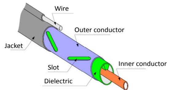
Fig. 1 Leaky Coaxial cable (LCX)
