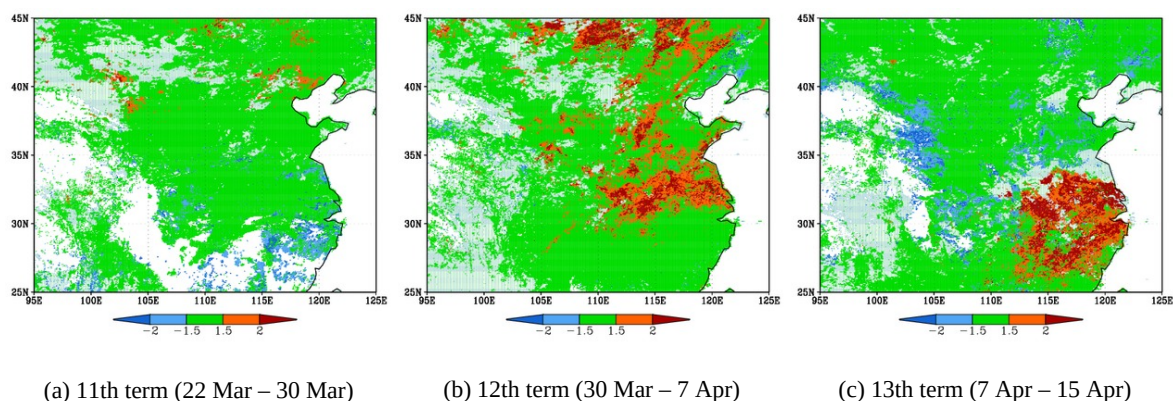
Fig. 9 Standard error of land surface temperature at night from 11th to 13th term derived from MOD11C1. In this figure, the region which has more than 2 degree standard deviation is vivid colored.
