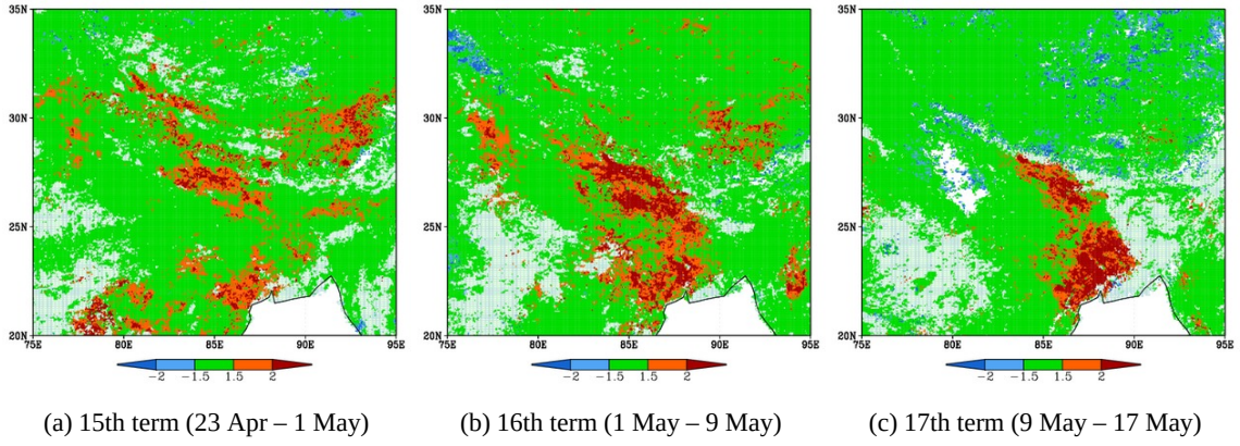
Fig. 11 Standard error of daily land surface temperature from 15th to 17th term derived from MOD11C1. In this figure, the region which has more than 2 degree standard deviation is vivid colored.
