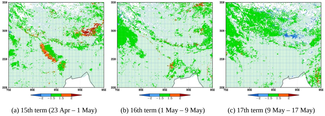
Fig. 12 Standard error of land surface temperature at night from 15th to 17th term derived from MOD11C1. In this figure, the region which has more than 2 degree standard deviation is vivid colored.
