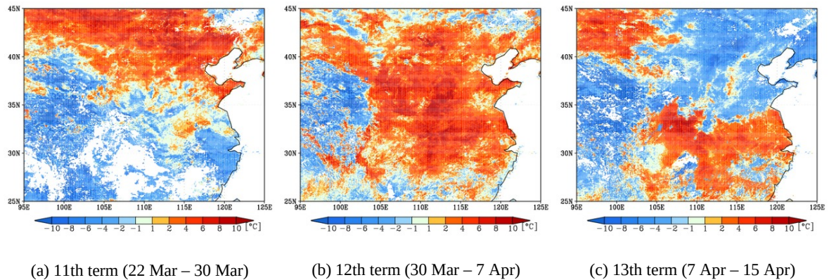
Fig. 8 Deviation of daily land surface temperature from 9 years average from 11th to 13th 2005 derived from MYD11C1
