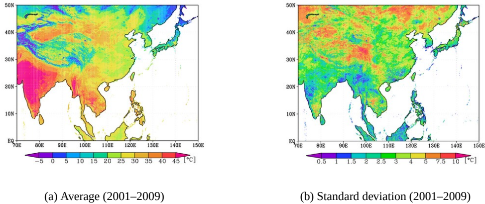
Fig. 2 Daily land surface temperature on 12th term.
