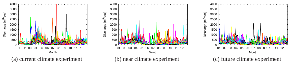
Fig. 13 Simulated discharge at Sagoshi (6,500km 2 ) in the Mogami River basin.
