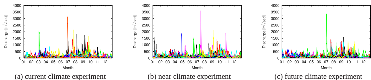
Fig. 14 Simulated discharge at Fukushima (3,171km 2 ) in the Abukuma River basin.
