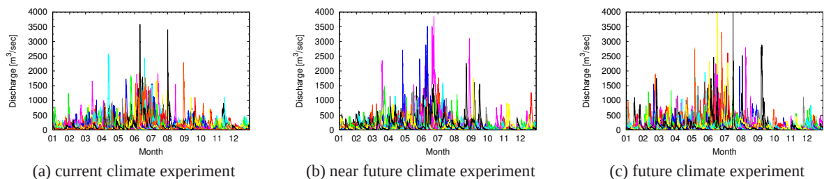
Fig. 16 Simulated discharge at Senoshita (2,315km 2 ) in the Chikugo River basin.
