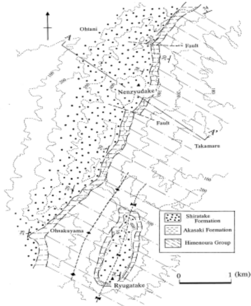
Fig. 2 Geological map
