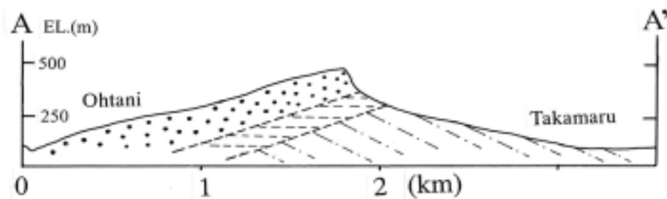
Fig. 3 Geological section
