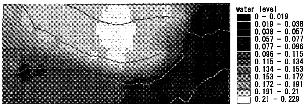
Fig. 4 Distribution of water table in the study area. The lowest ground level in the study area is defined as 0(m).
