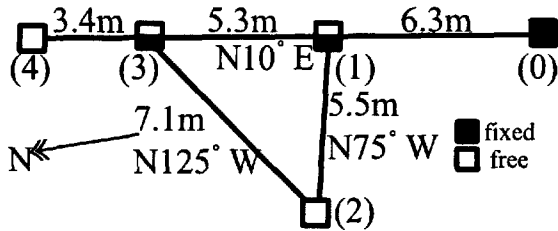
Fig. 3 Distribution of the displacement sensors of extensometers settled in the Osawa observation vault. Each numeral denotes the sensor number. (0) means the fixed end.
