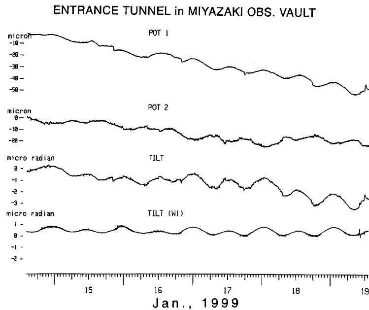
Fig.5 Record of test observation at entrance tunnel in Miyazaki observatory vault by type III instrument. (from top to bottom: POT1 level, POT2 level, tilt and record of routine tilt observation in the same direction in the observatory by type I instrument.)
