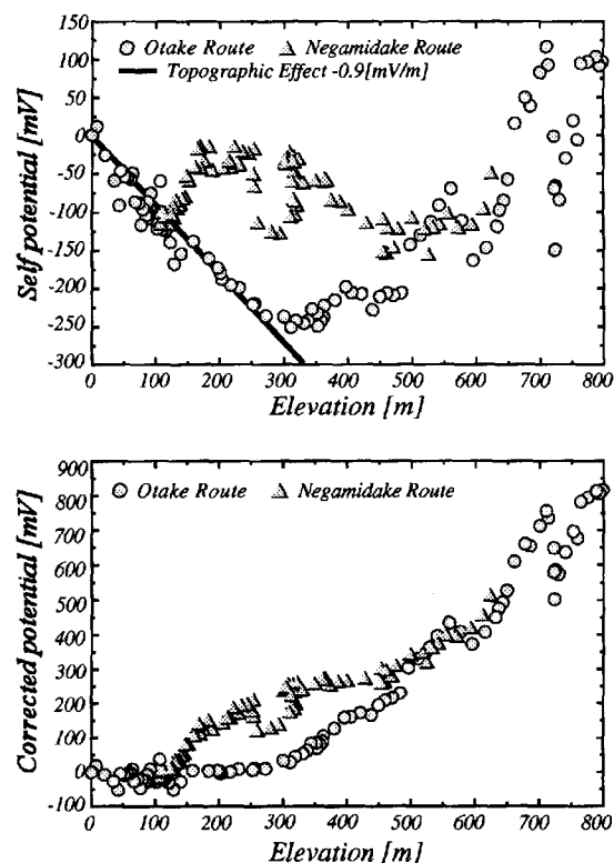
Fig. 4 Relation between topography (horizontal axis) and self-potential (vertical axis). Top panel shows the measured potential along two routes (circles and triangles). Thick line is a linear approximation for the data below 300 m altitude along the Otake route (-0.9 mV/m). Bottom panel shows the corrected potential by subtracting a linear topographic effect.
