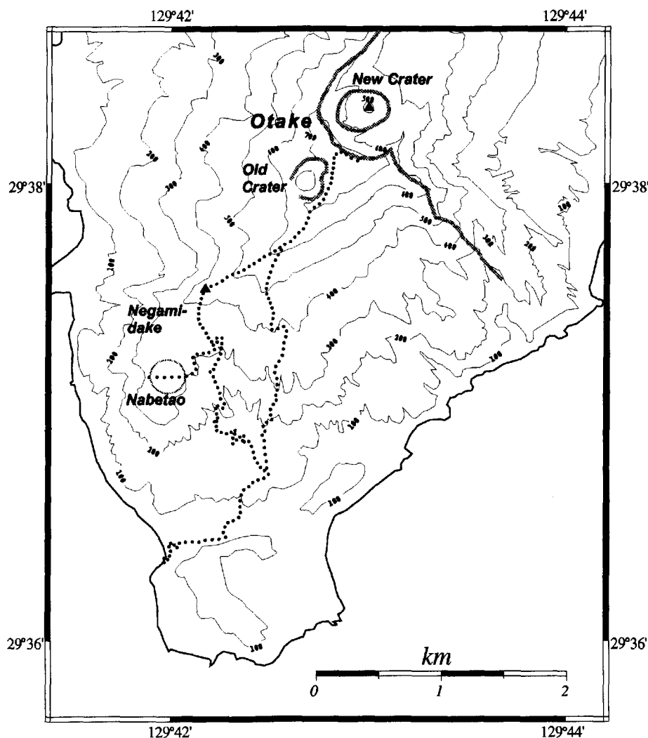
Fig. 2 Southern part of Suwanosejima island. Thick curve shows the outline of craters and the horse-shoe-shaped caldera. Measurement points of the self-potential survey in October 1998 are shown by black dots.
