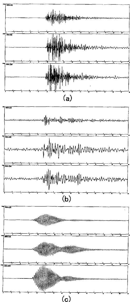
Fig.2 Examples of typical waveforms of volcanic earthquakes observed at Satsuma-Iwojima. (a) A-type earthquakes at 10:18 on January 17, 1999, (b) B-type earthquake at 23:35 on July 27, 1998 and (c) C-type tremor at 18:24 on July 10, 1998.
