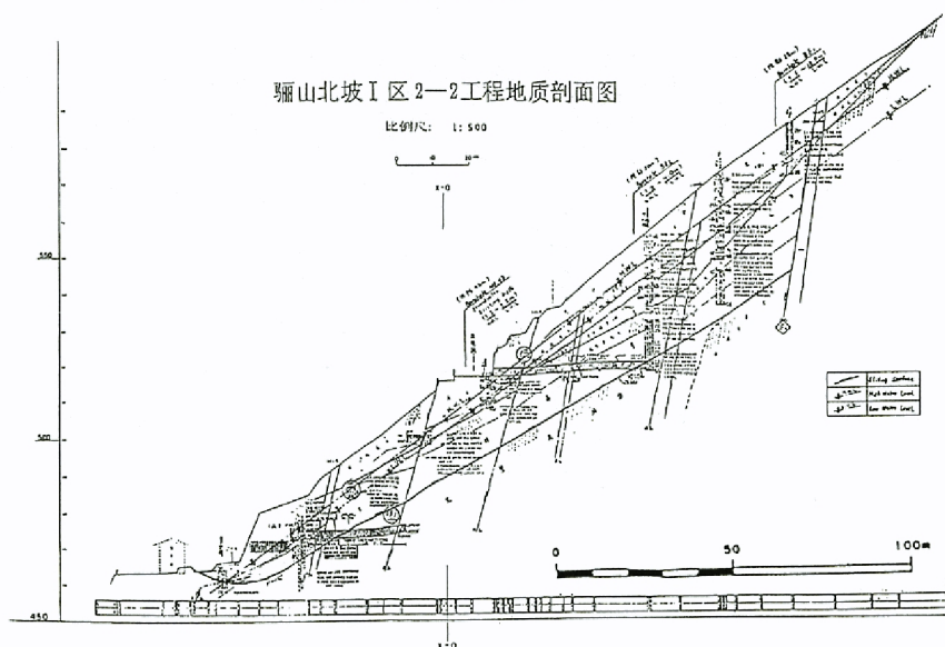
Fig 3 Analysis section of I Block
