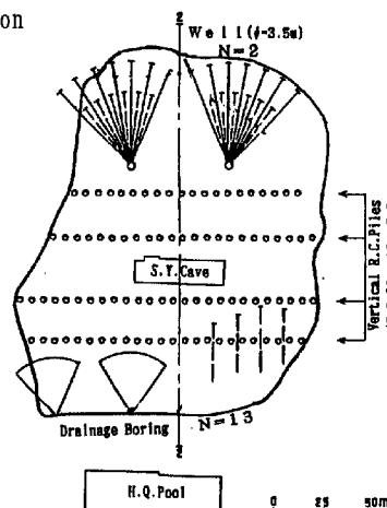
Fig. 9 Model of R.C. Piles
