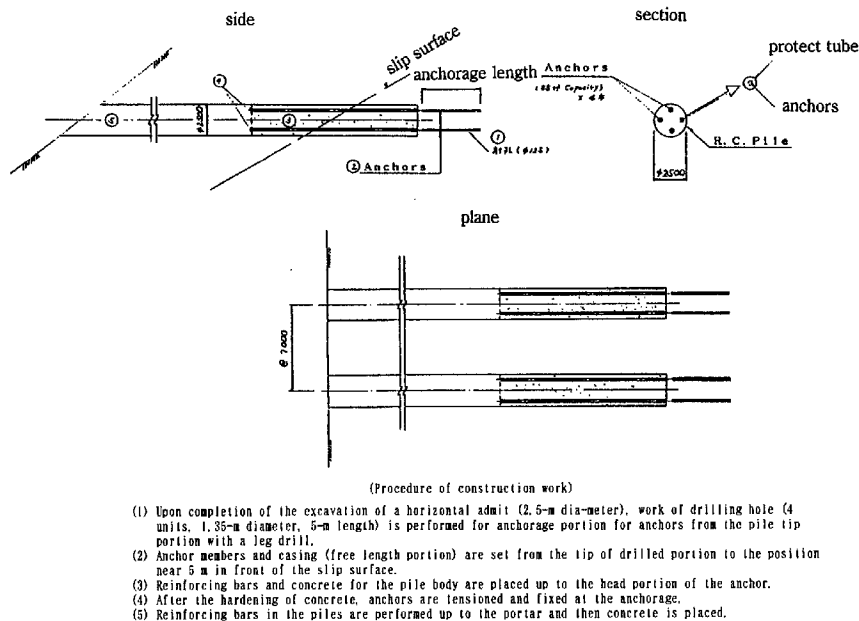
Fig. 14 Model of RC Piles+Anchors, CASE 1
