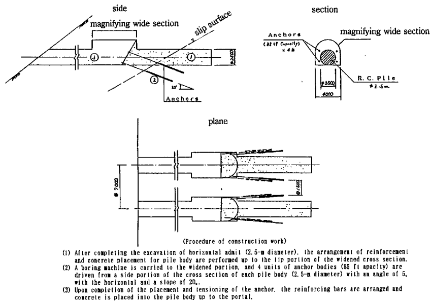
Fig. 14 Model of RC Piles+Anchors, CASE 1
