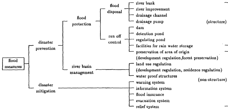
Fig.7 Idea of comprehensive flood control measures
