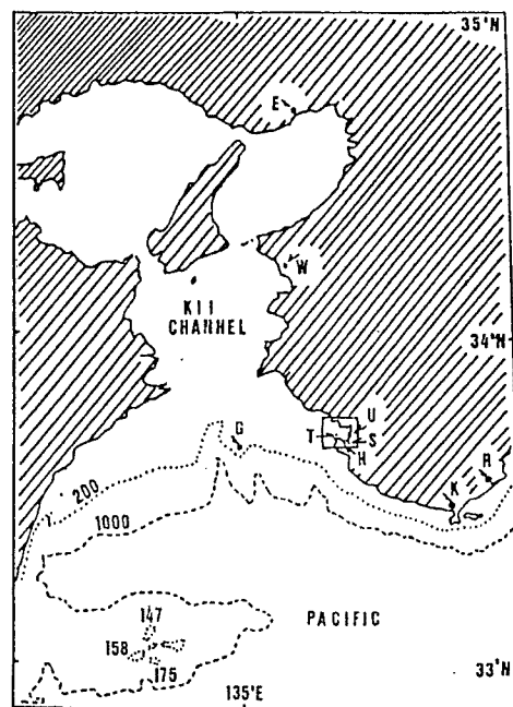
Fig. 1 Coastal and bathymetric conditions around the Shirahama Oceanographic Tower Station which is located offshore in the Northwestern Pacific.
