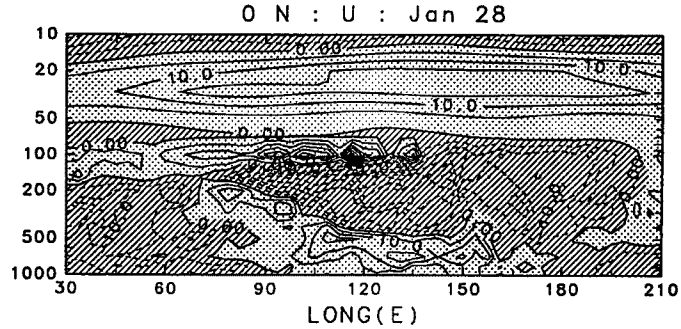
Fig. 2 Longitude ( ^{\circ} E)-height (hPa) section of the zonal wind (unit m/s) on 28 Jan. The contour intervals are 5 m/s. Dotted area is westerly and hatched easterly.
