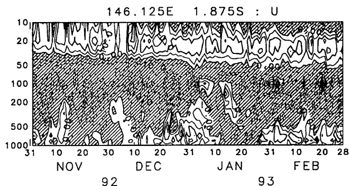
Fig. 1 Time-height (hPa) section of the zonal wind (unit m/s). The negative values (easterly) are shaded.
