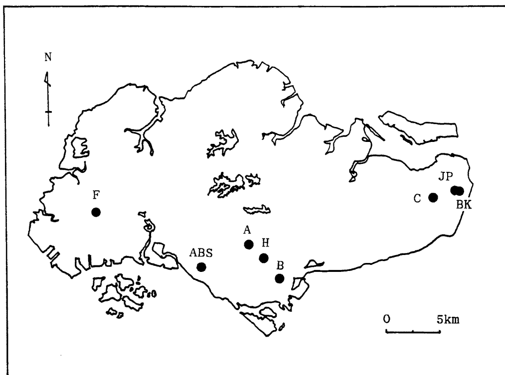
Fig. 1 Gravity Stations in Singapore.
