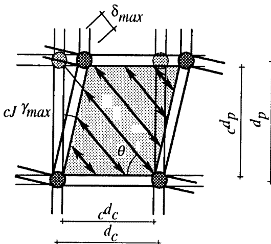
Fig. 14 Model of concrete panel.
