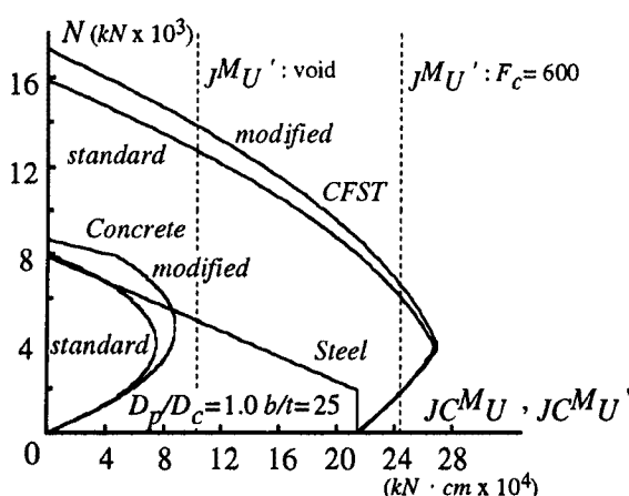
Fig. 7 N-M interaction curves.
