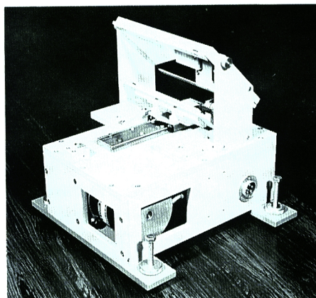
Photo. 2. The mirror system for light sheet shifting.
