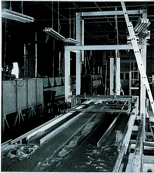
Photo. 1. A measurement carriage with coupled wheels.
