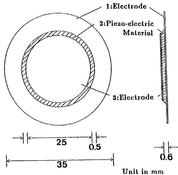
Fig. 2. Piezo-electric Oscillator.
