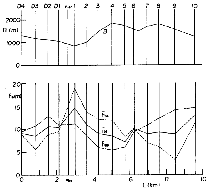
Fig. 16. Longitudinal variations of river width ( B ), mean water depth ( \bar{h}_s, \bar{h}_{sR}, \bar{h}_{sL} ) for total, right and left half sides of the cross-section of river channel at RL+6 m in water stage along the reach near Meghna Bridge.
