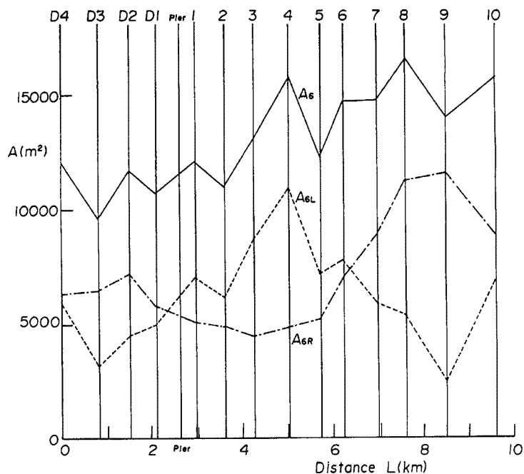
Fig. 17. Longitudinal variation of cross-sectional areas ( A_s, A_{sR}, A_{sL} ) for total, right and left half sides of the section of river channel at RL+6 m in water stage along the reach near Meghna Bridge site.
