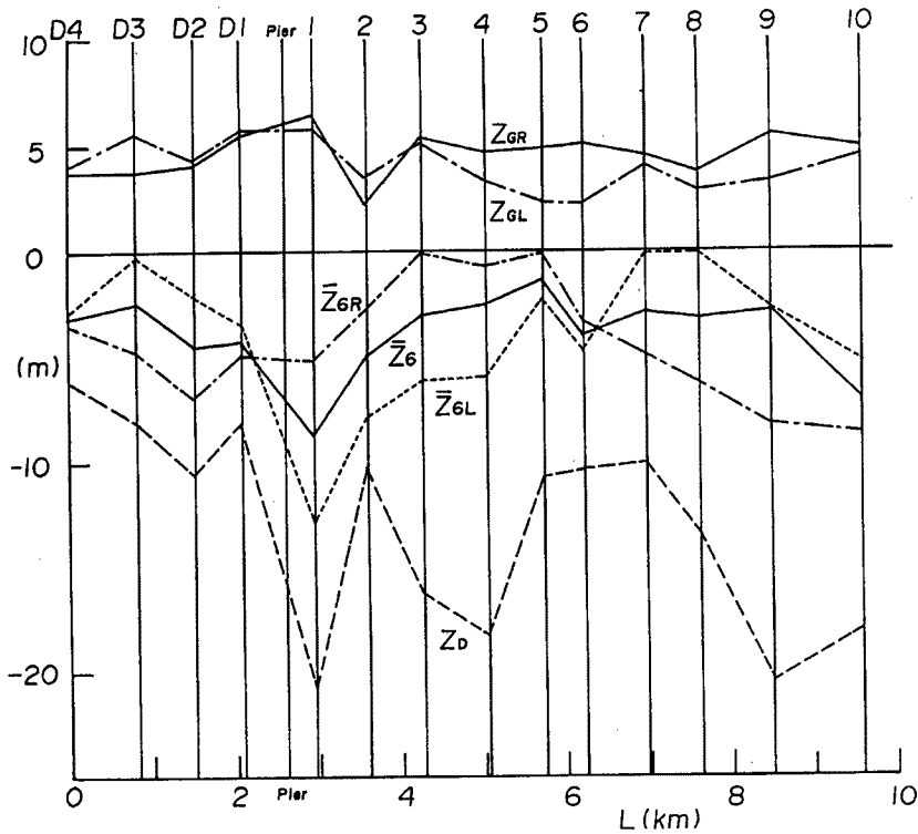
Fig. 15. Longitudinal profiles of ground levels of river bank ( Z_{GR} , Z_{GL} ) for right and left sides, mean bed levels ( \bar{Z}_s , \bar{Z}_{sR} , \bar{Z}_{sL} ) for total, right and left half sides of the cross-section of river channel at RL+6 m in water stage, and the lowest bed level ( \bar{Z}_D ) along the reach near Meghna Bridge.
