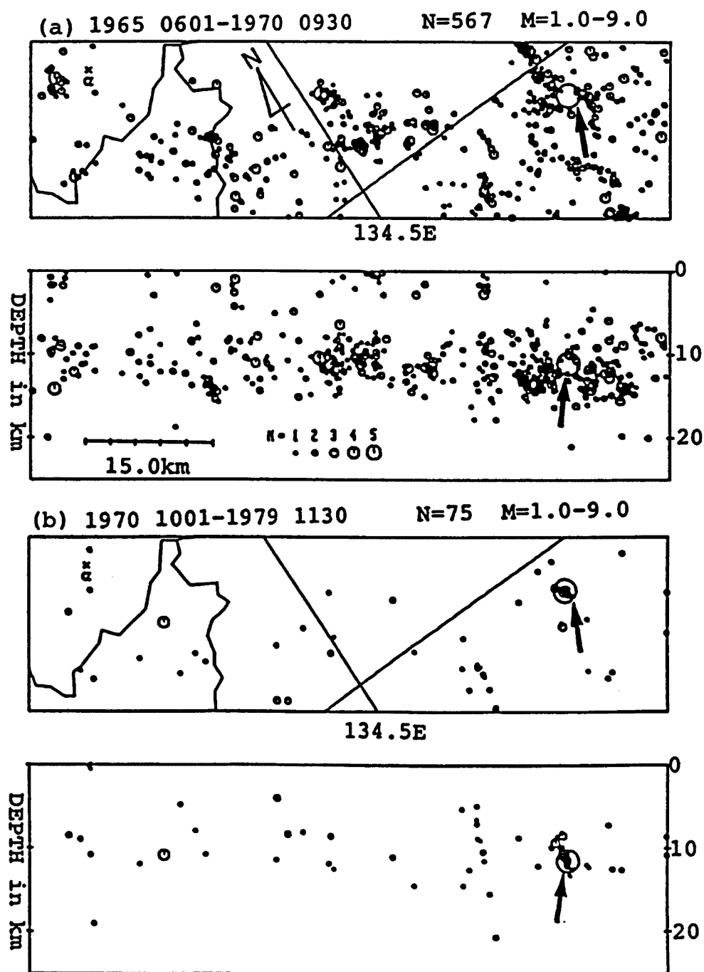
Fig. 14. Epicenter distribution (upper) and vertical cross section (lower) before and after swarm near Fukusaki (No.4 in Table2 and Fig.8). They are shown by being divided into two periods (a) and (b). Thick circles that are pointed out with arrows represent a focal area of the swarm.
