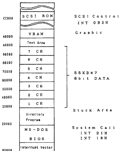
Fig. 4 Memory map of the CPU. Data area occupies 448 Kbyte from the address 30000H to 9FFFFH.
