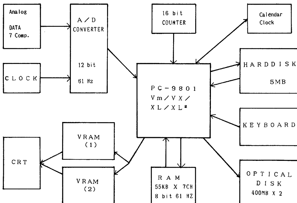
Fig. 1 Block diagram showing a continous observation system.
