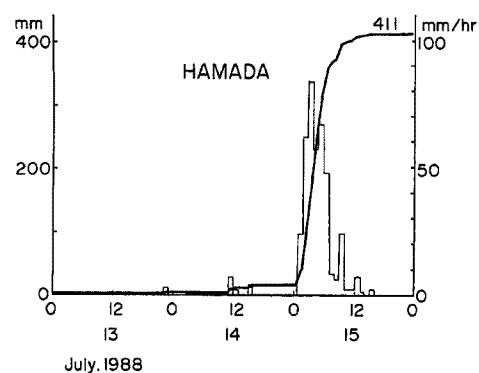
Fig. 4. Hyetograph.
