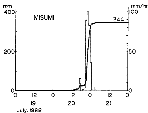
Fig. 5(a). Hyetograph.
