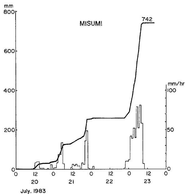
Fig. 3. Hyetograph.
