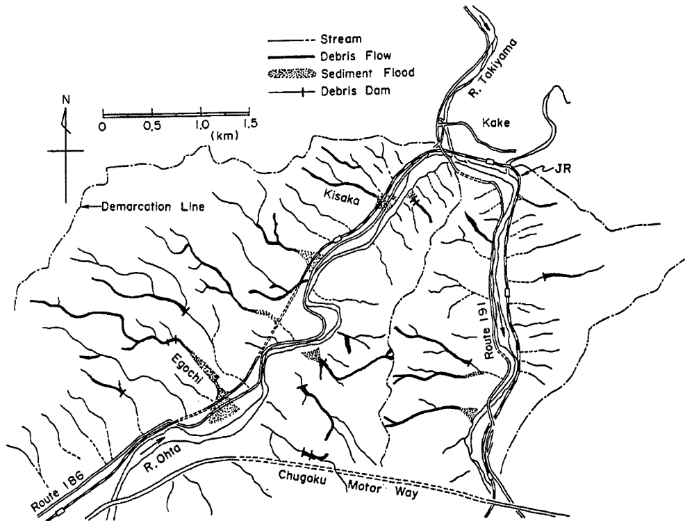
Fig. 14. Distribution of debris flows and slope failures in Kake Town.
