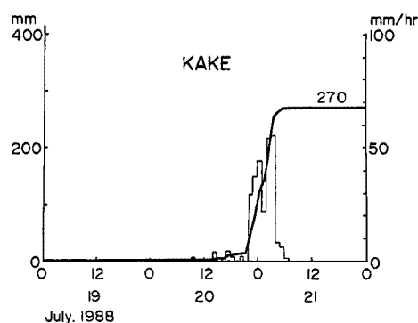
(b). Hyetograph.
