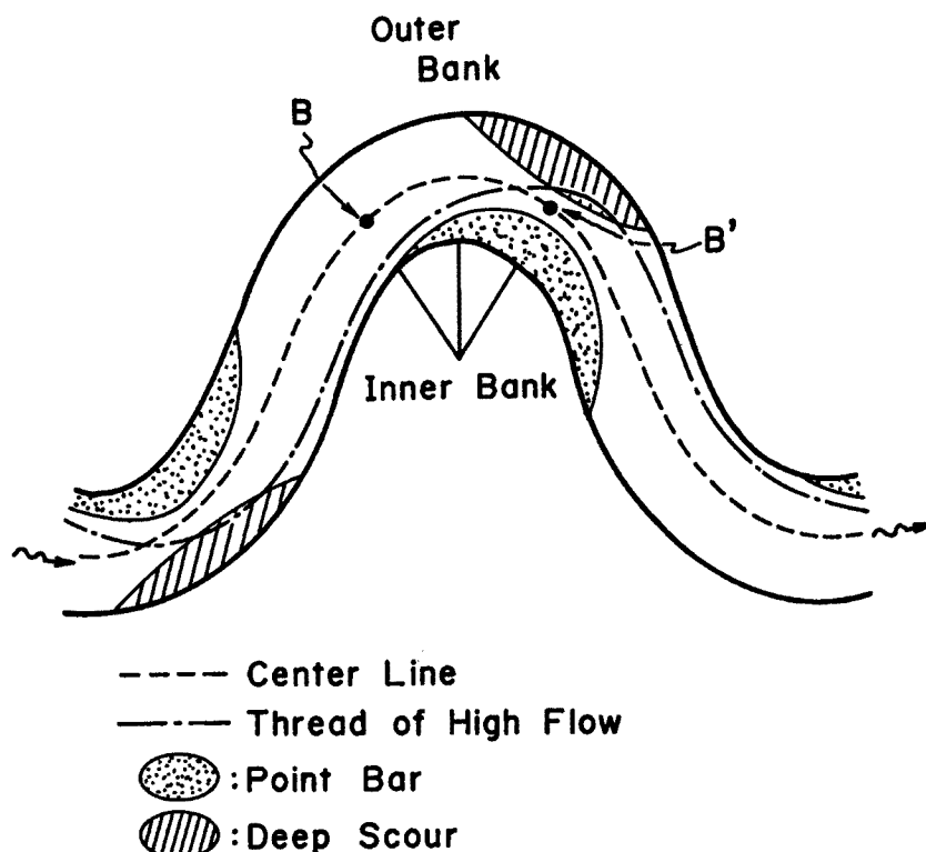
Fig. 3. Meandering channel
