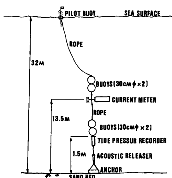
Fig. 2 Schema of mooring system for current observation.
