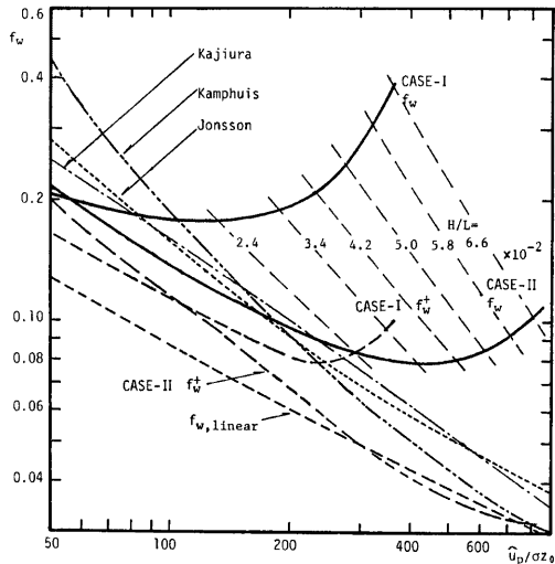
Fig. 7 Comparisons of calculated results of friction factor with those by existing formulas.
