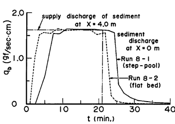
Fig. 4 Sediment discharges transported on the armoured flat bed (Run 8-2) and on the armoured bed with step-pool (Run 8-1).
