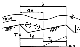
Fig. 17 Schematic of shear stress distribution along the step-pool bed surface.
