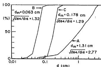
Fig. 2 Sand particle sizes used in flume experiments.
