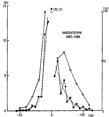
Fig. 2 Frequency distribution (black circle) and accumulated amount (open circle) of the daily change of snow depth at Hakodateyama
