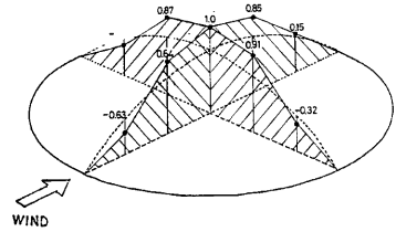
Fig. 11 Mean displacement of membrane
