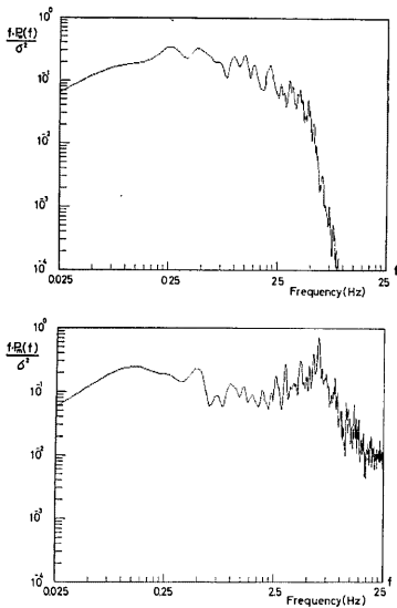
Fig. 8 Power-spectral-density function of dynamic pressure and membrane displacement (at point3)
