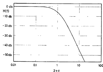
Fig. 3 Frequency characteristics of digital filter H(f)
