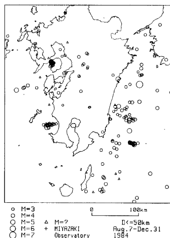
Fig. 6 Epicenter distribution of shallow earthquakes occurred after the main shock in the southern and eastern areas of Kyushu (JMA). Epicenters of aftershocks are omitted.
