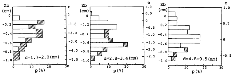
Fig. 3 Distribution of the bottom height and degree of exposure of tracer particles
