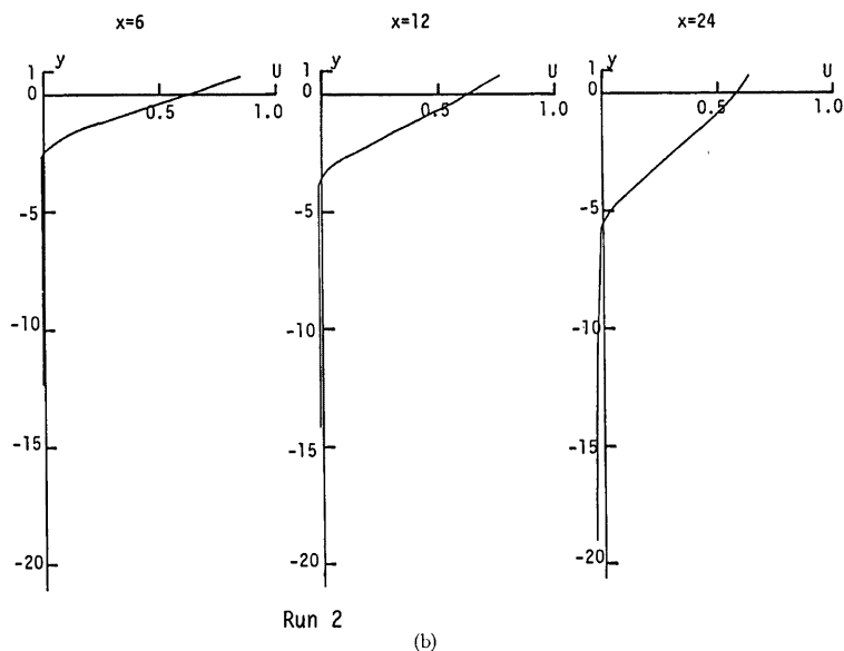
Fig. 15 (a), (b) Velocity distribution
