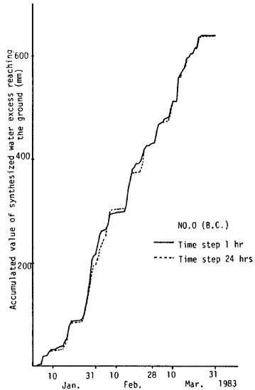
Fig. 23 Synthesized water excess reaching the ground surface for various computation intervals
