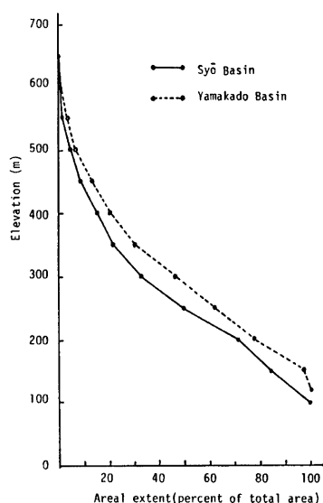
Fig. 2 Relationship between elevation and areal extent
