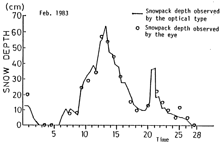
Fig. 4 Comparison between the snowpack depths observed by the eye and by the optical snowpack meter at B.C. point
