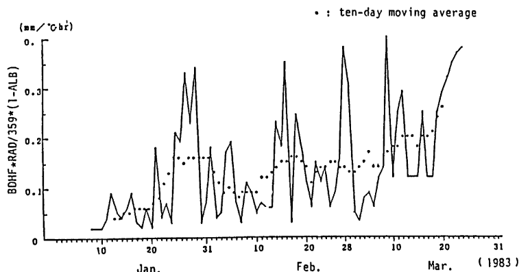
Fig. 10 Daily variation of snowmelt factor BDHF \cdot RAD / 359 \cdot (1 - ALB)
