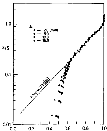
Fig. 6 Mean wind speed profiles above urban model: x = 10.9 m ( x_1 = 1.3 m)
