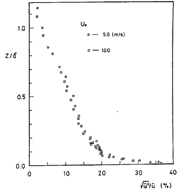
Fig. 12 Turbulence intensity profiles above urban model: x=9.7 m ( x_1=0.1 ).
