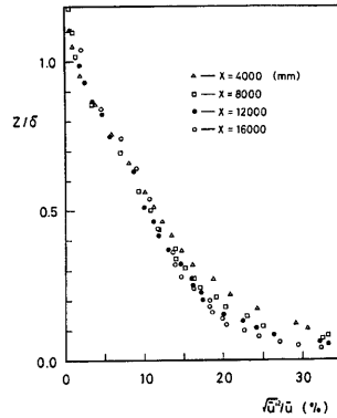
Fig. 14 Turbulence intensity profiles above artificial grasses: U_0=10.0 m/s.
