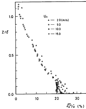
Fig. 11 Turbulence intensity profiles above urban model: x=10.9 m ( x_1=1.3 m).
