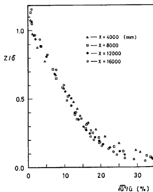
Fig. 13 Turbulence intensity profiles above artificial grasses: U_0=5.0 m/s.
