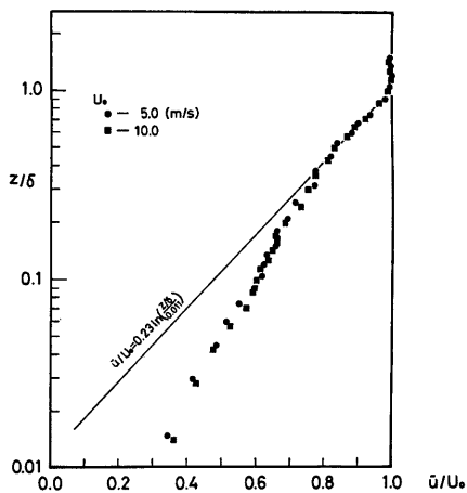
Fig. 7 Mean wind speed profiles above urban model: x = 0.7 m ( x_1 = 0.1 m)
