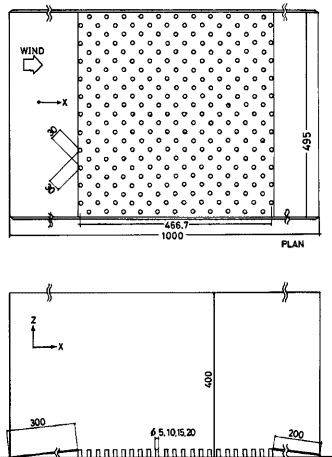
Fig. 1 Arrangement of roughness plate
