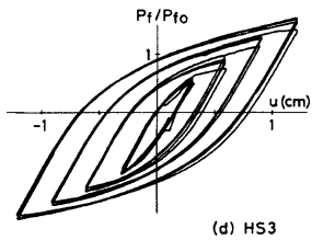
Fig. 7 P_f/P_{fo}-u relationships (HS series)
