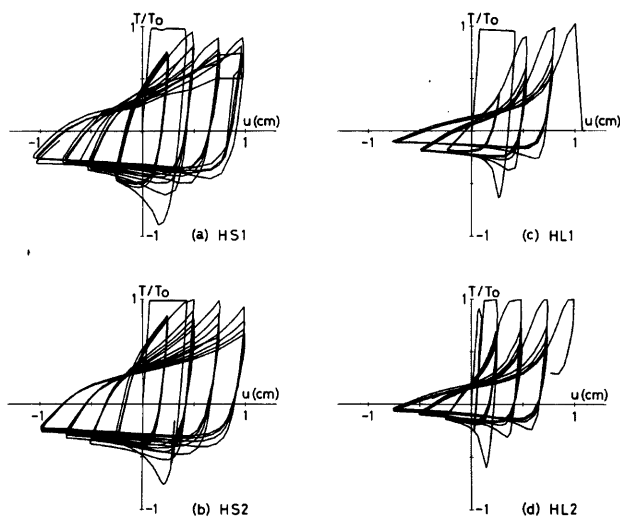
Fig. 11 T/T_0-u relationships.
