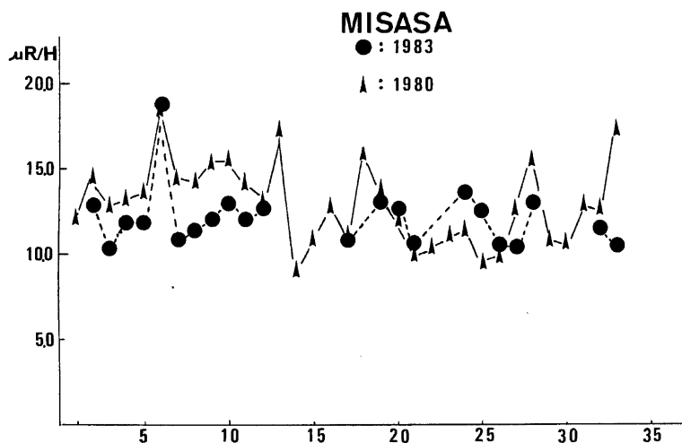
Fig. 1 The relation between the results of the \gamma -ray intensities in 1980 and them in 1983 in the Misasa area is shown. The vertical axis indicates the observation values in \mu\text{R}/\text{H} and the horizontal one indicates the numbers of the observation points. Both of the results are similar each other.
