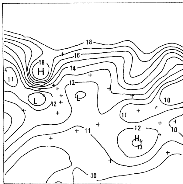
Fig. 3 The map shown by the contours. The pattern of the distribution of the \gamma -ray intensities has not changed since 1980.
