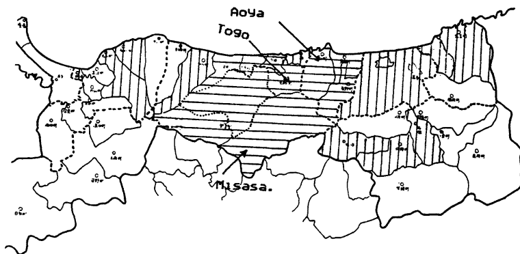
Fig. 8 The distribution of the seismic intensities in the Tottori prefecture
