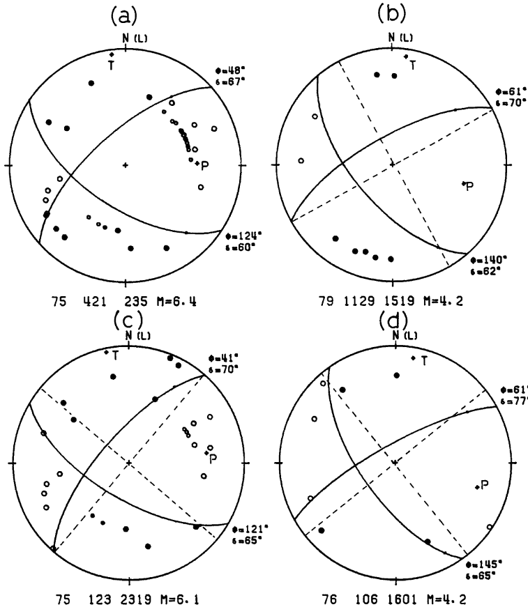
Fig. 8 Fault plane solutions for events in Fig. 7
