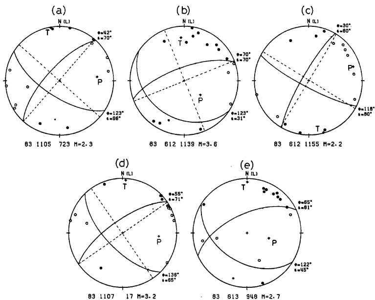
Fig. 5 Fault plane solutions for events in Fig. 2. All represent the lower hemispheres of equal area projections. Solid symbols are compressions and open symbols are dilatations. The solid curve indicates the nodal line of the assumed normal fault type, and the broken line indicates the strike slip type solution.
