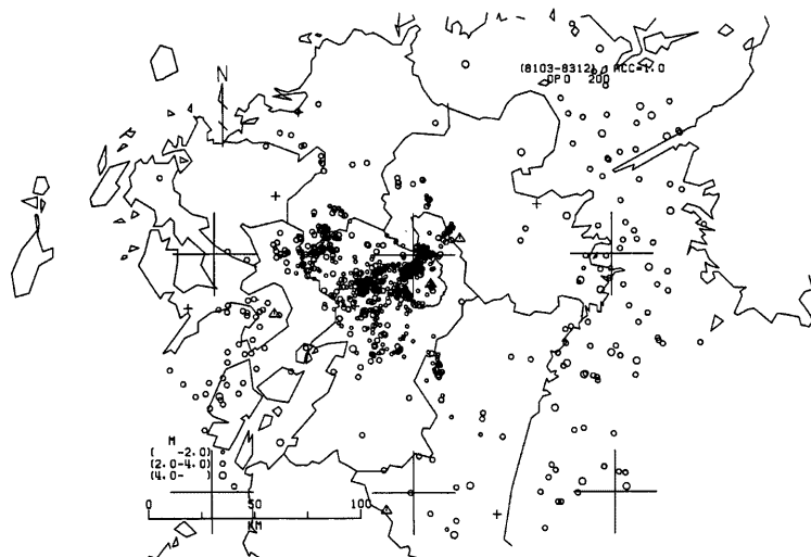
Fig. 1 Distribution of epicenters for well-located events in the central Kyushu during period 1981 to 1983. Locations have been calculated by the seismic network of AVL (Aso Volcanological Laboratory, Kyoto Univ.). The active seismic region is shown in the western part of the central Kyushu. Dense clusters of events near the Aso Caldera have been discussed in Fig. 2. Small cross symbols are the main cities in each prefectures. Small triangles are the active volcanoes; Unzen, Aso, Kuju and Kirishima.
