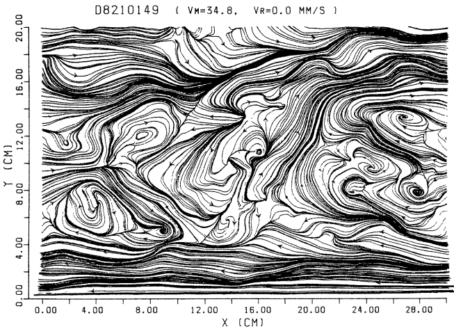
Fig. 8 Patterns of steramlines viewed by the observer moving at a speed equivalent to the mean velocity of the flow field. The case of frame No. 149.
