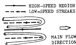
Fig. 19 Spatial distribution of horse-shoe vortex, high-speed region and low-speed streaks.
