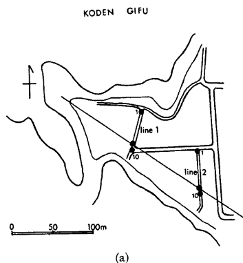
Fig. 4. a. Survey route at Koden area in the Neo fault. b. Results of the survey along lines 1 and 2.
