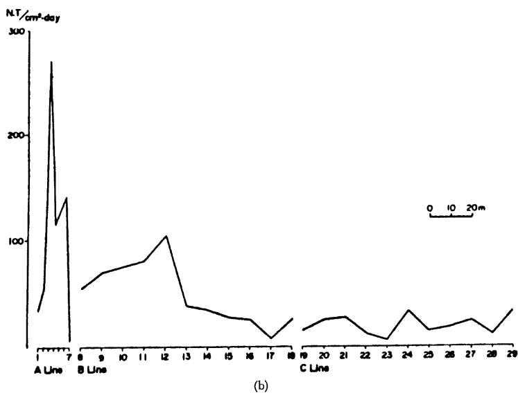
Fig. 13. a. Location of the Tanna fault. b. Result of the survey of a track by Geological Survey of Japan.
