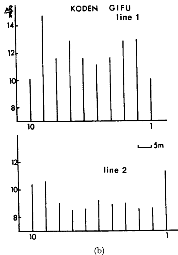
Fig. 4. a. Survey route at Koden area in the Neo fault. b. Results of the survey along lines 1 and 2.
