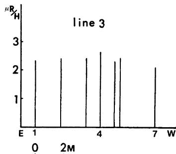
Fig. 12. Results of the survey at the Tanna fault along lines 3.
