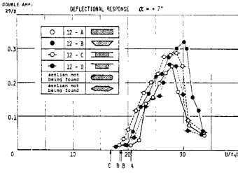
Fig. 6. Velocity-Amplitude Curve.
