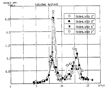
Fig. 13. Velocity-Amplitude Curve.
